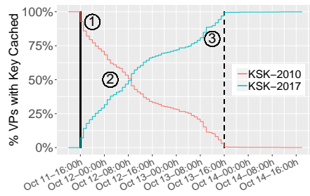
Figure 7: Key transition for all VPs.
