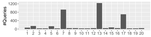
Figure 16: DNSKEY queries for root during experiments.
