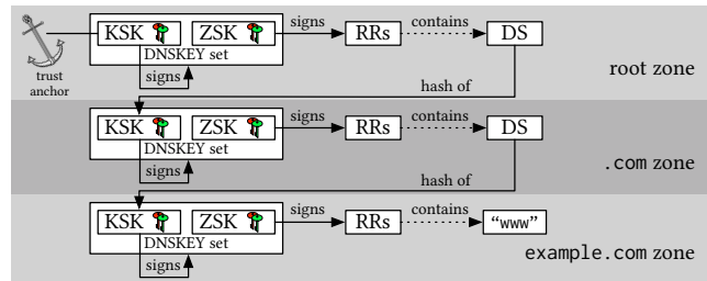
Figure 1: DNSSEC chain of trust, starting at the root.
